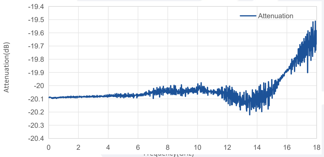
Attenuation vs Frequency
