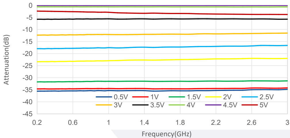
Attenuation@Voltage Pin=0dBm
