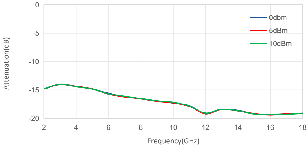
Attenuation@Pin V_T=2V
