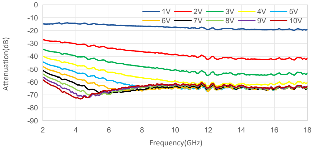
Attenuation@Voltage Pin=10dBm
