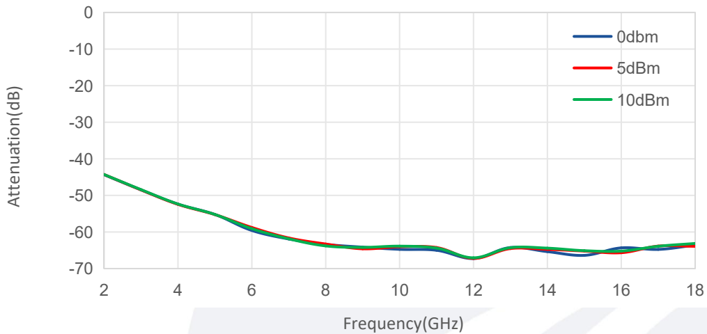
Attenuation@Pin V_T=6V
