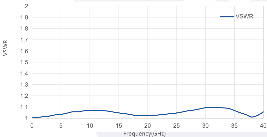
VSWR vs Frequency
