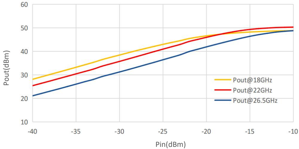
Pout@Equal_Pin
