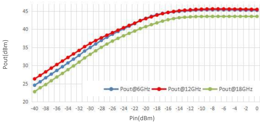
Pout@Equal_Pin
