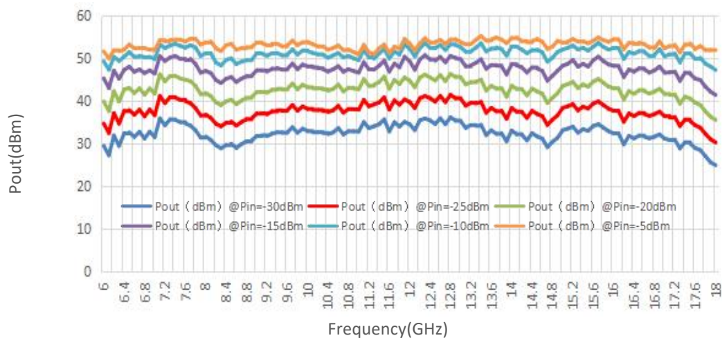
Pout@Equal_Pin
